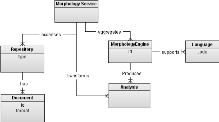
Morphology Service Entity Relationship Diagram
